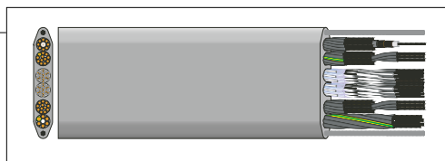
Flat cables FL, FM, FH and module concept, PVC and Low Fire Hazard
